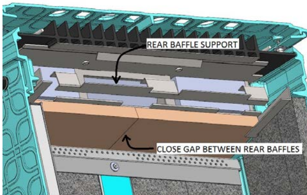
Figure 17 - Removing/Replacing the Rear Baffle for Inspection
