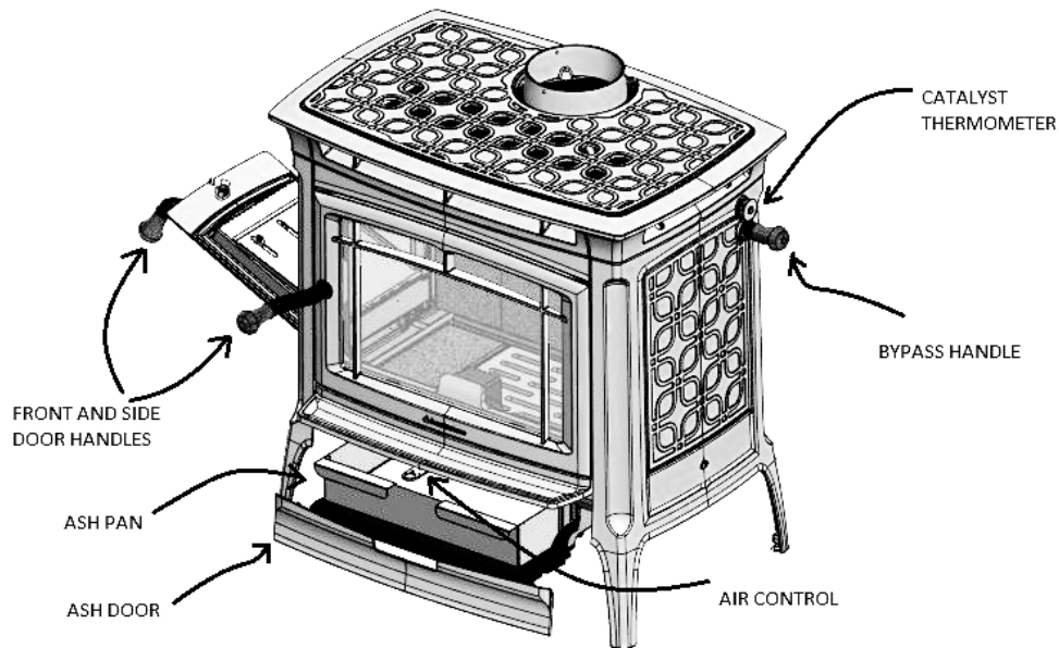
Figure 10 - Controls & Features
