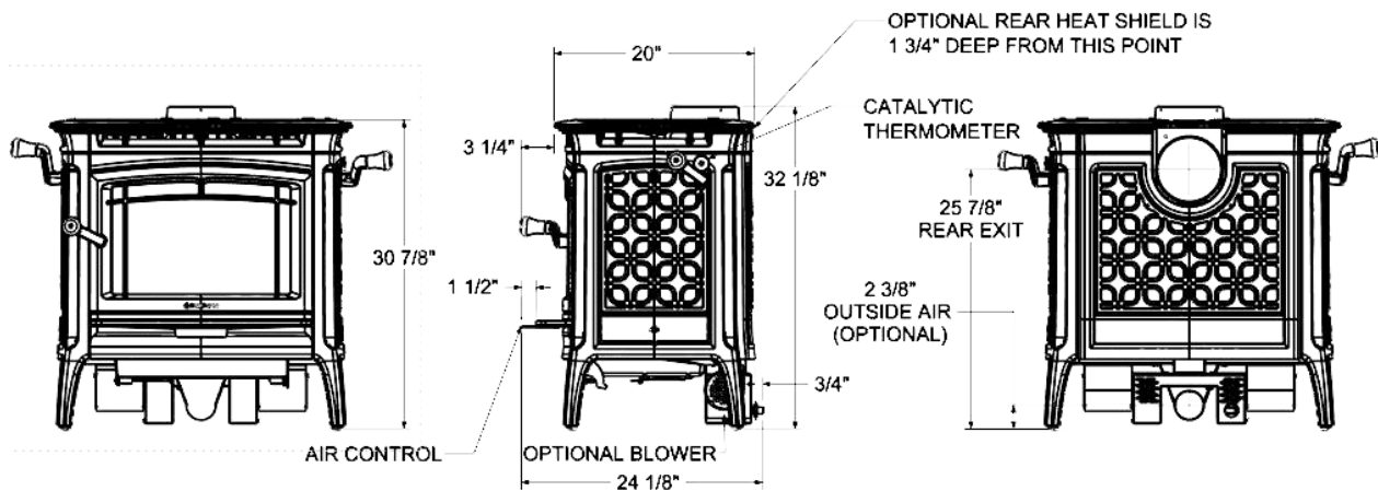
Figure 1 – Manchester 8362 Dimensions
